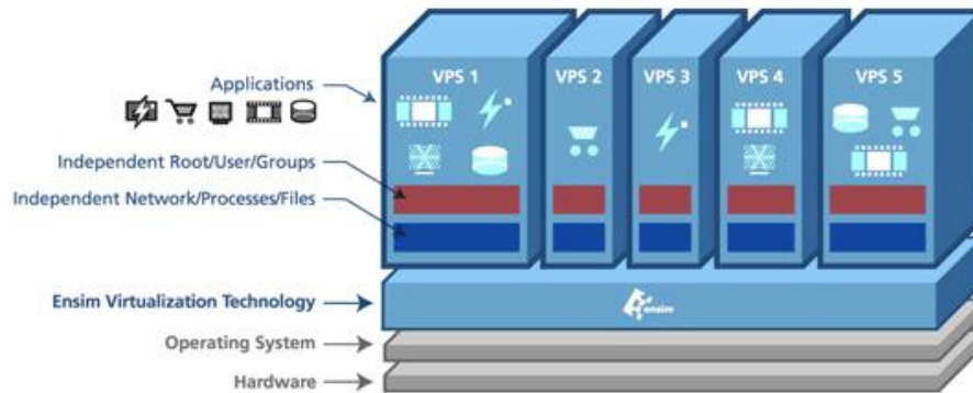
Figure 8: Ensim Virtual Private Server Architecture.
