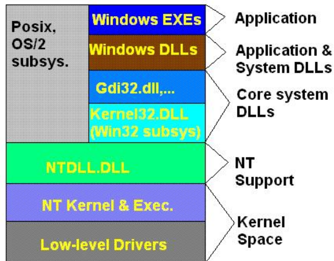
Figure 10: Windows NT Architecture.
