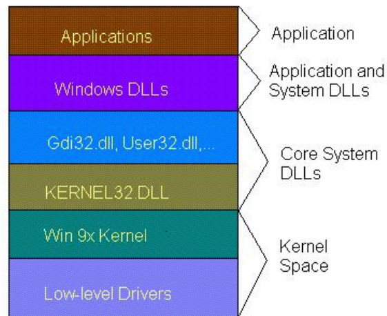
Figure 9: Windows 9x Architecture.
