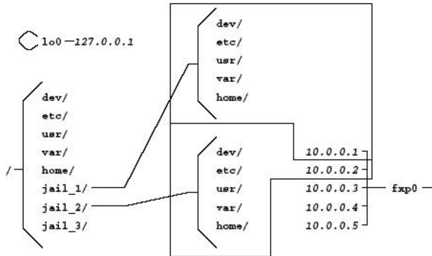
Figure 7: Machine with two configured jails.
