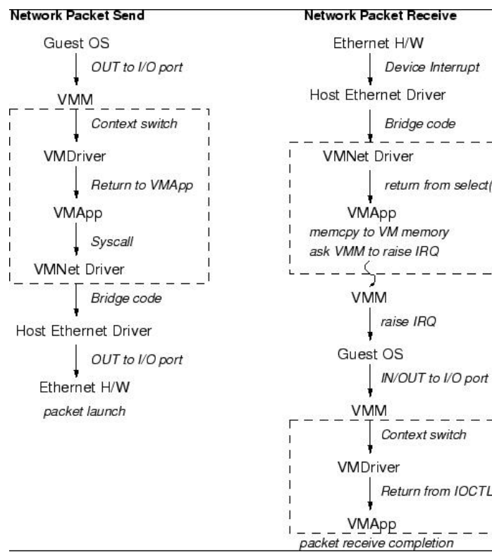
Figure 6: VMware Network Architecture.
