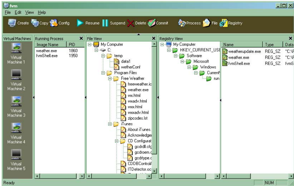
Figure 12: Graphical user interface of FVM showing permitted operations and properties.
