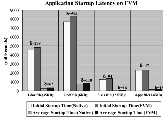
Figure 16: The startup latency for invoking four Windows applications in a new FVM virtual machine
