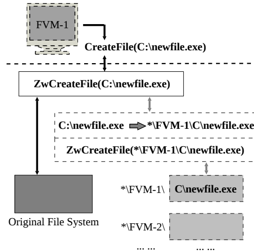
Figure 13: File system virtualization works by renaming file path name arguments at file open time in a way similar to registry entry renaming.
