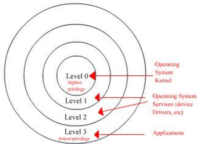
Figure 4: Intel x86 protection rings.
